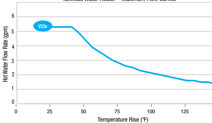
Tankless Water Heater – Maximum Flow Curves
